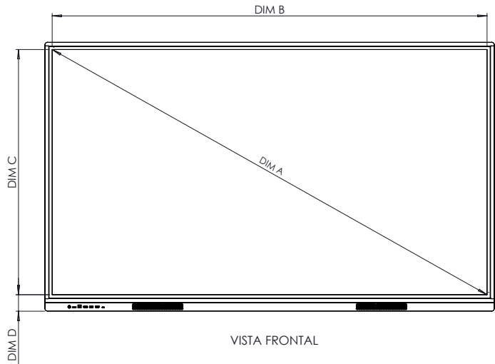
Vista frontal
